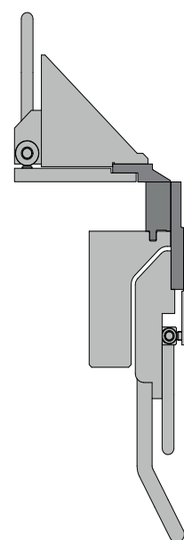
Lateral cut: sharp nose blade 20°/30° respectively radius blade R 2/3/4/5
